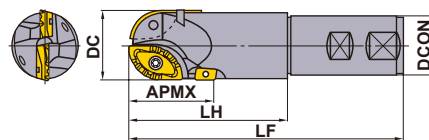
● Attachement Weldon (Fig.4)
